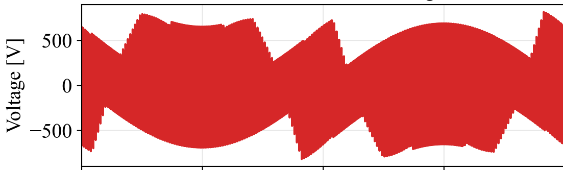
Inverter-side inductor voltage
