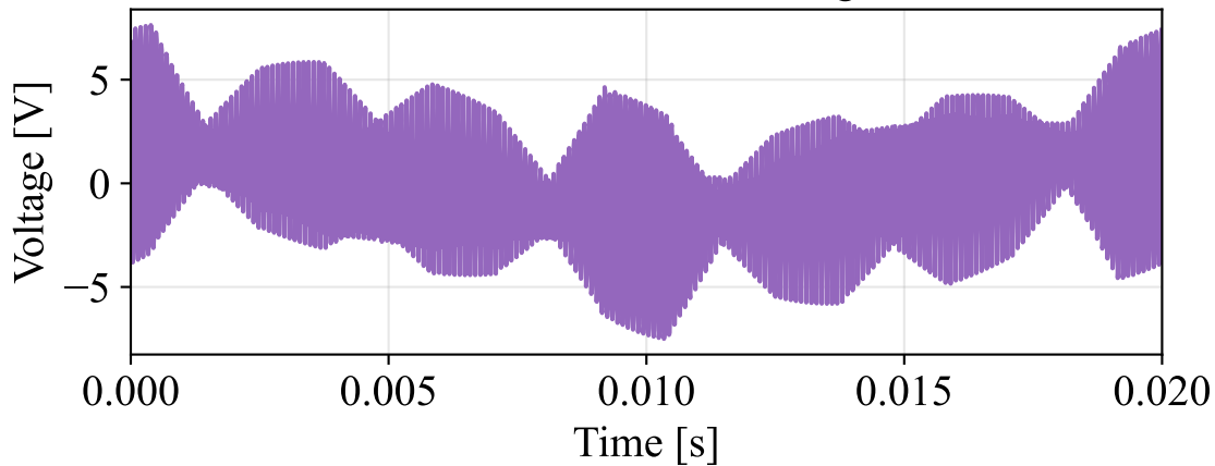
Grid-side inductor voltage
